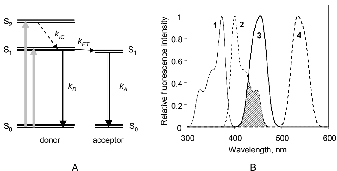
Figure 1.8. Simplified scheme of energy levels (Jablonski's diagram) for the donor-acceptor pair (A) and schematic normalized spectra for donor and acceptor (B). In figure (A) S_0 denotes the ground states of donor and acceptor, S_{1,2} – excited states, k_{IC} corresponds to the rate of internal conversion, k_D , k_A – donor and acceptor sum relaxation rates, k_{ET} – the rate of energy transfer. In figure (B) curves 1 and 2 represent the absorption and emission spectra of the donor; 3 and 4 are the absorption and emission spectra of the acceptor. The donor-acceptor spectral overlap area is indicated via hatching.
