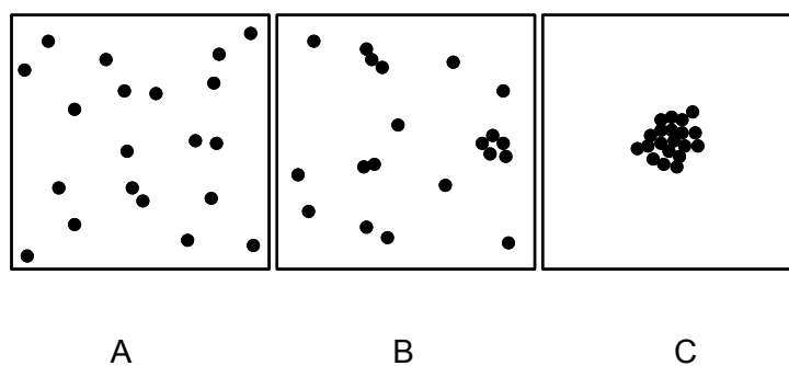
Figure 2.2. Schematic illustration of the effect of protein association resulting from the model described in the text. (A) Random distribution of proteins with k = 0 , (B) partially associated proteins with k = 0.5 , (C) completely associated proteins ( k = 1 ). Proteins are schematically indicated by solid dots. The figures show that at increasing values of k the proteins aggregate into clusters in a non-specific way.
