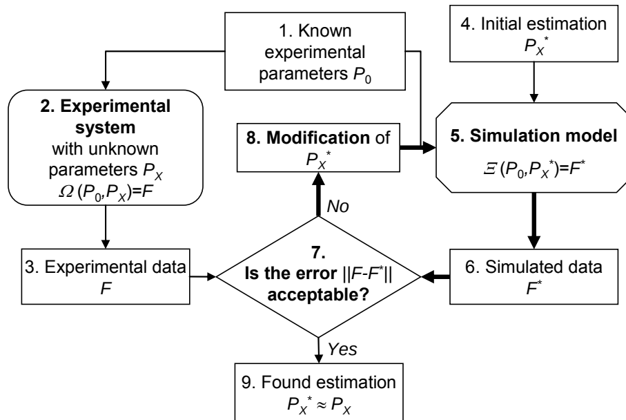
Figure 4.1. Flow diagram, demonstrating simulation-based fitting approach (see text). The thick line shows the fitting loop.
