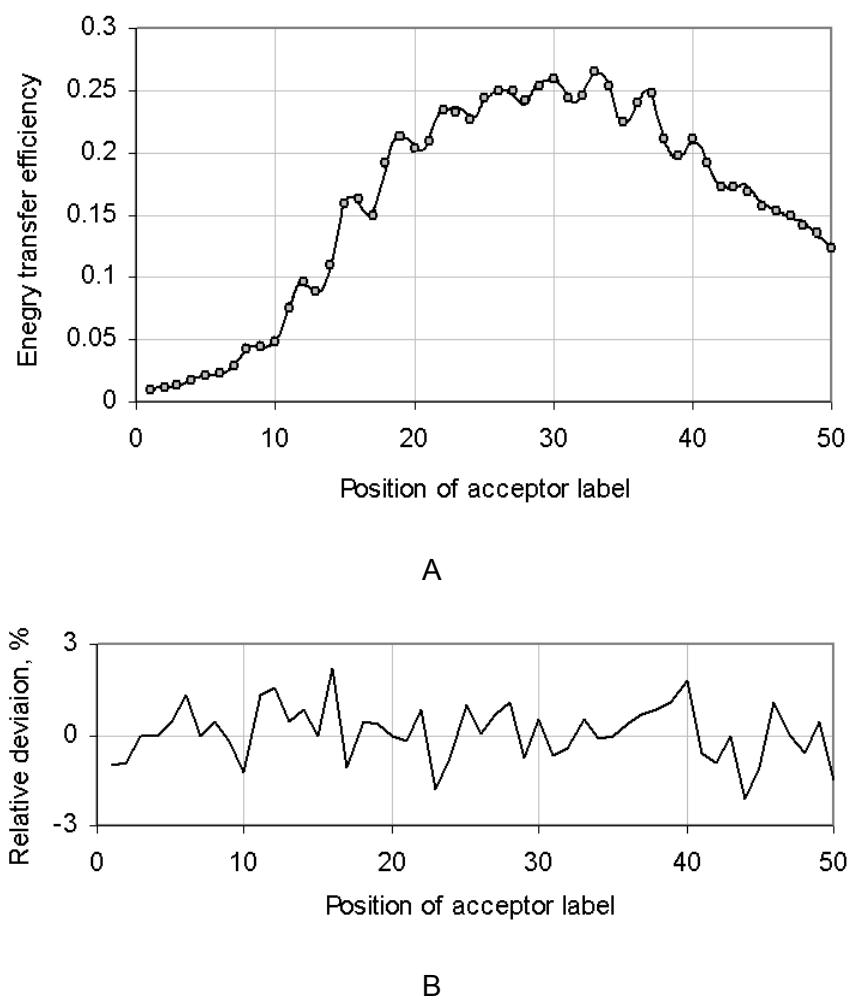
Figure 4.6. ANN approximation of the simulation model (A) and relative deviations of the ANN result and the simulation model (B). In (A) the circles show the result of the simulation modeling and the line is the ANN approximation.
