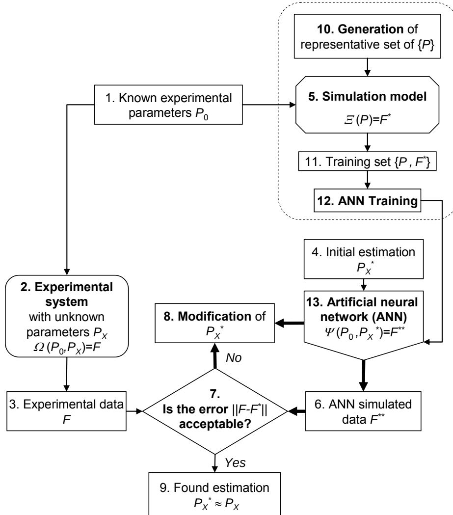
Figure 4.2. Flow diagram of simulation-based fitting with artificial neural network approximation. The dotted box shows the extension of the simulation-based fitting method (see Fig. 4.1) by the artificial neural network fitting procedure.
