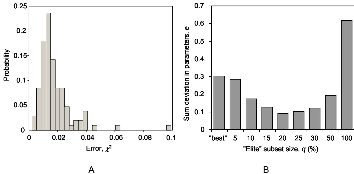
Figure 2.7. (A) Distribution of \chi^2 of the solutions found after 100 runs of SBF on experimental data and (B) behavior of the sum parameter deviation e (Eq. 2.28) with respect to the “elite” subset size q . The result in (B) is obtained after averaging the results of three independent numerical simulations. For all of them the optimal q was around 20%.
