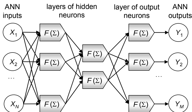
Figure 1.4. Example of a multilayer perceptron with N inputs ( X_i ), M outputs ( Y_j ) and three layers.
