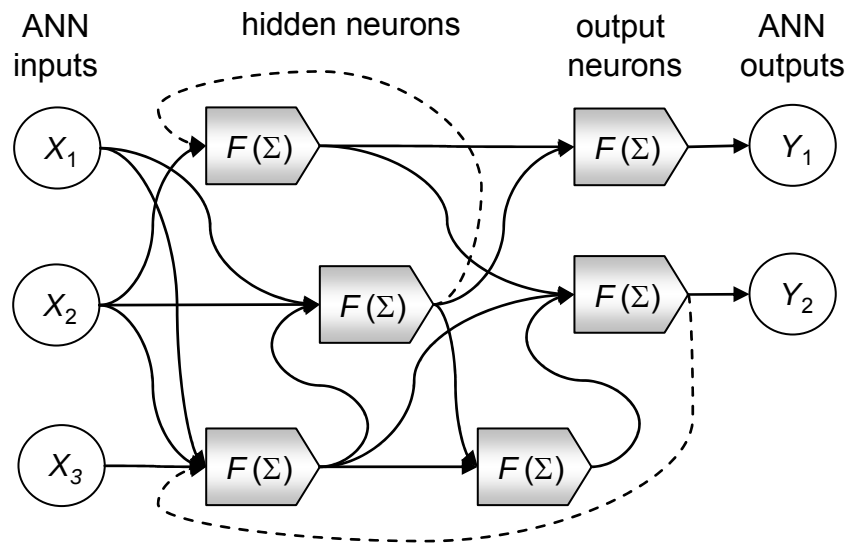
Figure 1.3. ANN with three inputs ( X_i ) and two outputs ( Y_j ). Feedback connections are marked by dotted lines.
