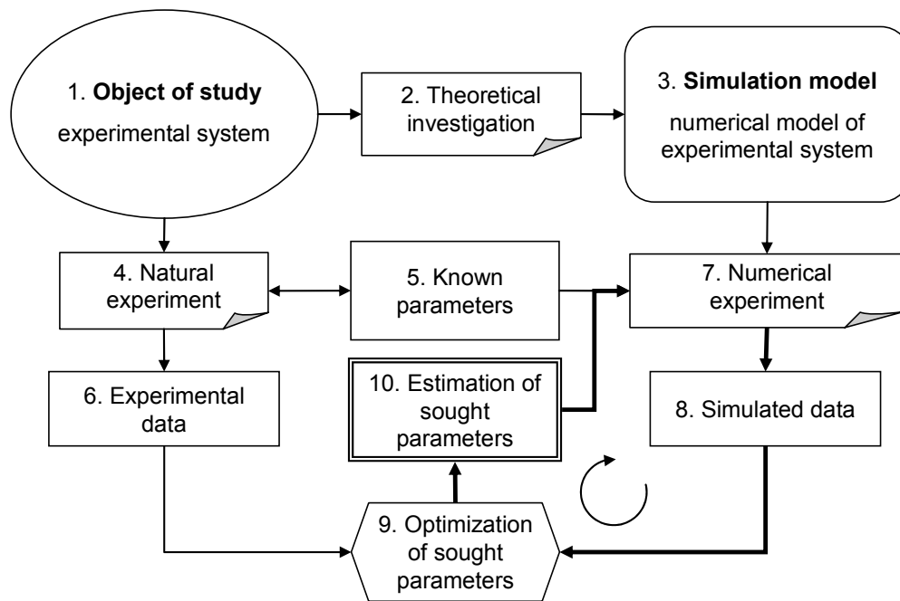
Figure 1.1. General solution of an inverse problem by the simulation-based fitting approach. Thick lines show the loop of the iterative estimation of the parameters sought.
