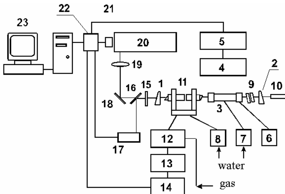
Figure 5.1. Intracavity laser spectrometer: 1 - output cavity mirror, 2 - back cavity mirror, 3 - dye laser, 4 - laser power supply, 5 - laser control unit, 6 - dye pump, 7 - laser water pump, 8 - atomizer water pump, 9 - Fabry-Perot interferometer, 10 - He-Ne laser, 11 - atomizer, 12 - atomizer gas supply, 13 - atomizer power supply, 14 - atomizer control unit, 15 - attenuator, 16 - beam splitter, 17 - photodiode, 18 - mirror, 19 - cylindrical lens, 20 - high-resolution spectrograph, 21 - CCD-camera, 22 - optical multichannel analyzer, 23 - PC.
