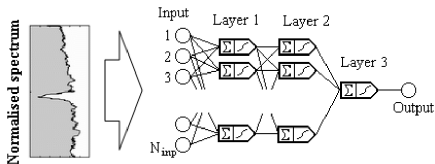
Figure 5.5. Three-layer feed-forward neural network (MLP) for analysis of normalized spectrum.
