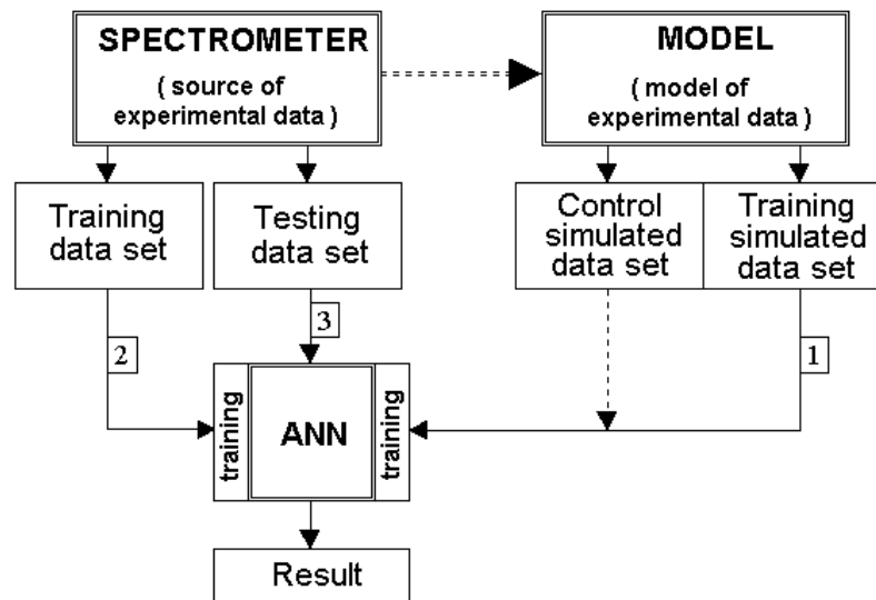
Figure 5.7. The algorithm of ANN training in the case of lack of experimental data.
