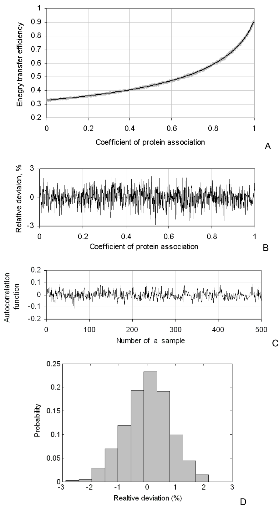
Figure 4.7. Consistency of the ANN approximation. In (A) the thick gray line is the result of the simulation modeling and the thin black line is the ANN approximation. Below this graph the relative deviations between simulation model and approximation (B) and their autocorrelation function (C) are given. The distribution of deviations is given in (D).
