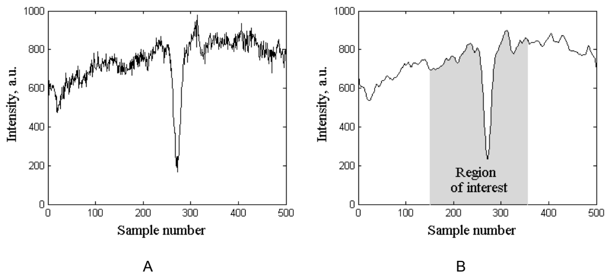
Figure 5.4. High frequency noise cancellation by Fourier filtration: (A) – initial spectrum, (B) – filtered spectrum.
