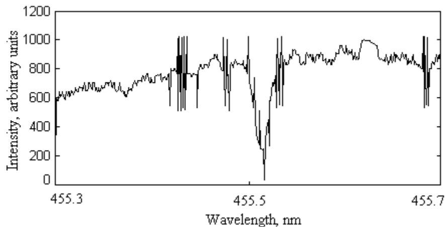
Figure 5.2. Raw absorption spectrum of Cs (narrow gap) on top of the laser pulse spectrum
