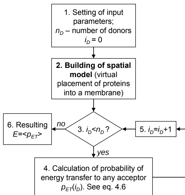
Figure 4.5. Flow diagram of a single simulation of energy transfer in a protein-lipid system.
