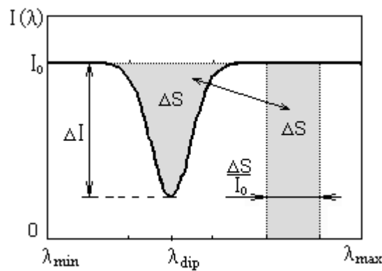
Figure 5.3. Parameters of absorption spectra: relative depth of the gap \Delta I/I_0 and area \Delta S/I_0
