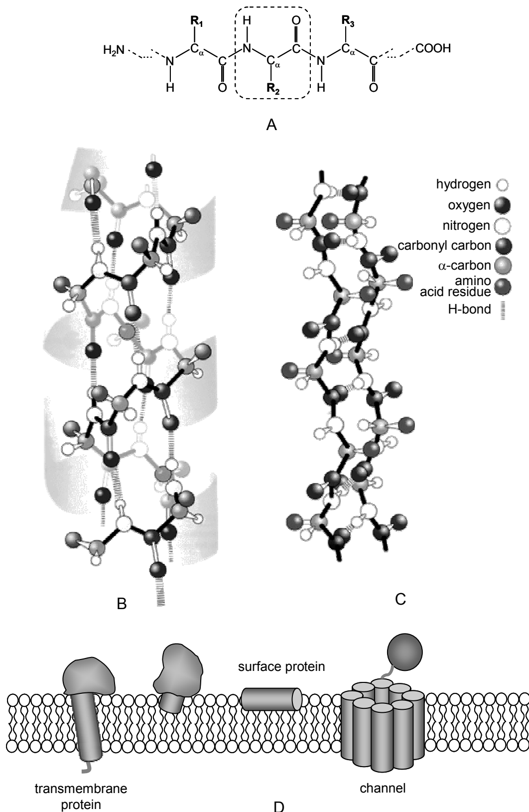
Figure 1.6. Polypeptide link in a protein (A), and two ordered secondary structures of proteins: \alpha -helix (B) and \beta -sheet (C) conformations (Devlin, 2006). Different types of membrane protein incorporation into a membrane (D).
