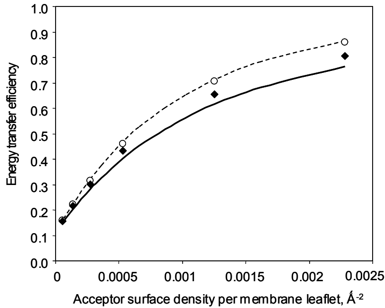
Figure 2.6. Comparison of simulation results with analytical solutions for different sizes of proteins. Solid line: analytical result for D_P = 10 Å; ♦: simulation results with the same protein exclusion distance D_P = 10 Å; dotted line: analytical energy transfer efficiency; o: simulated energy transfer efficiency for D_P = 1 Å. All calculations were performed with the following protein parameters: n_A = 46 , n_D = 26 , \theta = 16^\circ , \psi = 50^\circ , d = 10 Å, S_L = 72 Å 2 , and R_0 = 24 Å. The corresponding parameters for the analytical model are: h_I = 26.8 Å, h_{II} = 13.1 Å, and R_{intra} = 33.9 Å.
