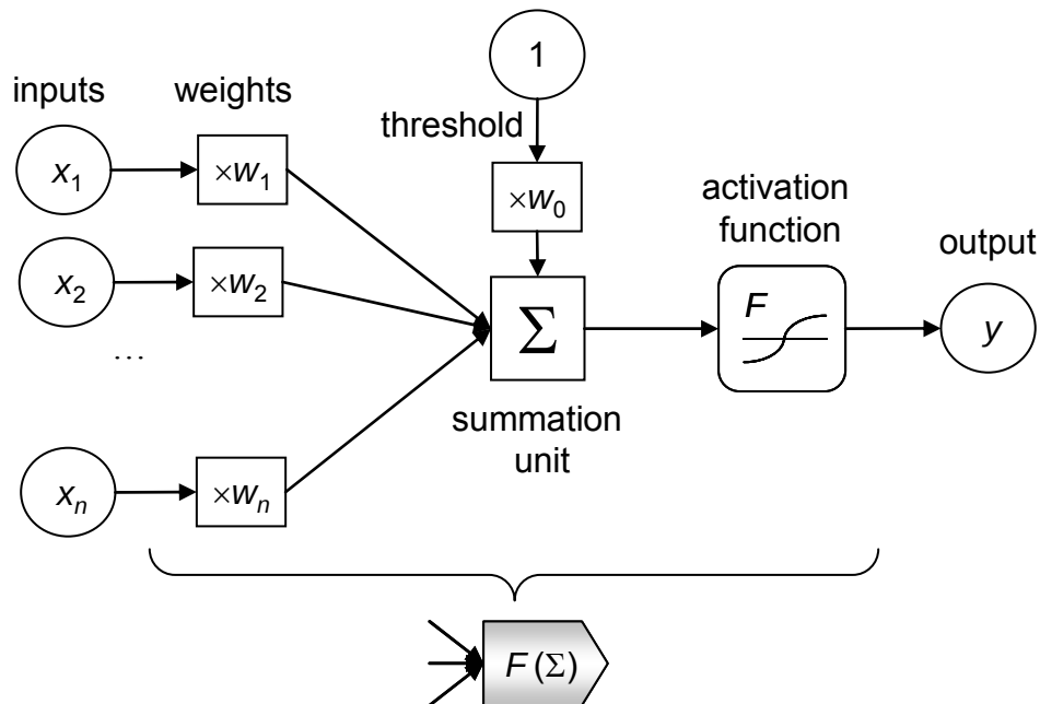
Figure 1.2. Classical artificial neuron with n inputs ( x_i ) and weight factors ( w_i ), threshold ( w_0 ), non-linear activation function F and the symbolic notation of an artificial neuron (at the bottom).
