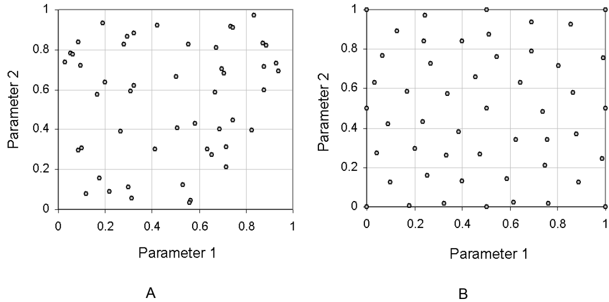
Figure 4.3. Illustration of the principle of point selection in a two-dimensional parameter space. Uniformly distributed random points are shown in (A). Points obtained by the proposed algorithm are presented in (B).
