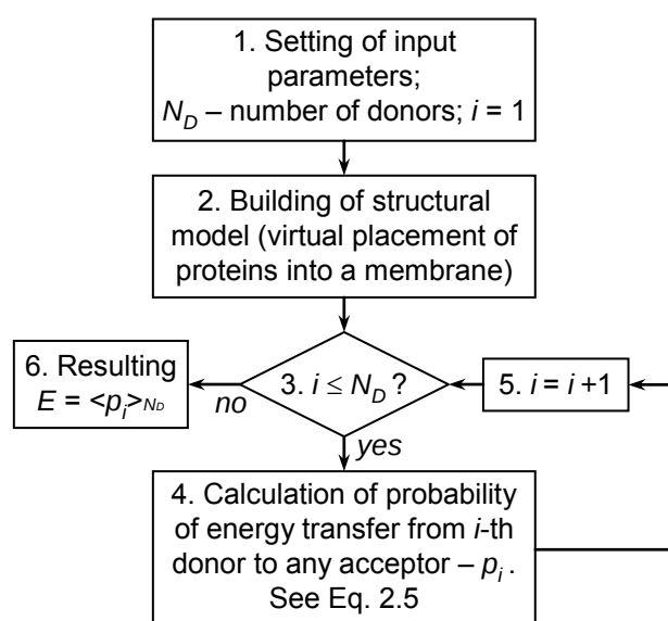
Figure 2.3. Flow diagram of a single simulation of energy transfer in a protein-lipid system.
